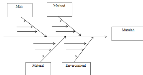
Gambar 1. Diagram Fishbone
