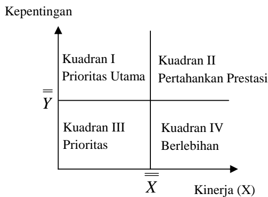
Gambar 1. Diagram Kartesius
